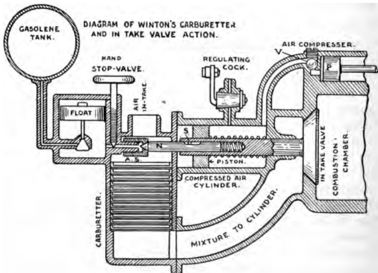
FIG. 216.—Diagrammatic Sketch of Winton's Carburetter and Intake Valve Action, as applied to a Horizontal Cylinder Engine.
